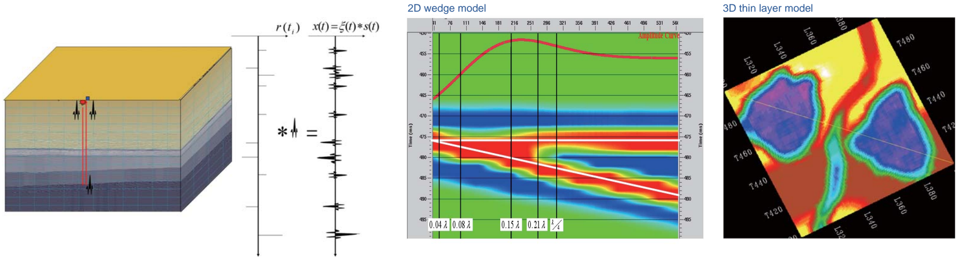
Reflectivity
