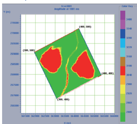
Thin-bed reservoir
