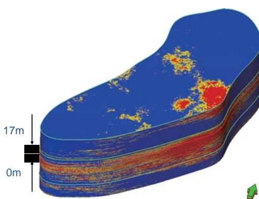
Thin-bed reservoir
