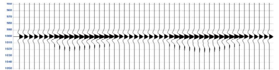
3-8-35-45(0°) band-pass wavelet
